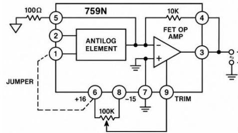
Figure 5. Trimming E_{OS} in Antilog Mode
