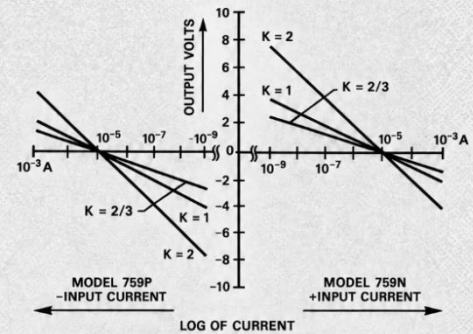
Plot of Output Voltage vs Input Current for Model 759 Connected in the Log Mode
