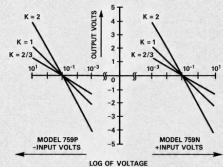
Plot of Output Voltage vs Input Voltage for Model 759 Connected in the Log Mode
