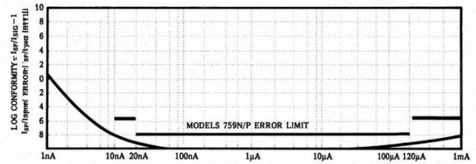
Figure 2. Log Conformity Error for Models 759N and 759P
