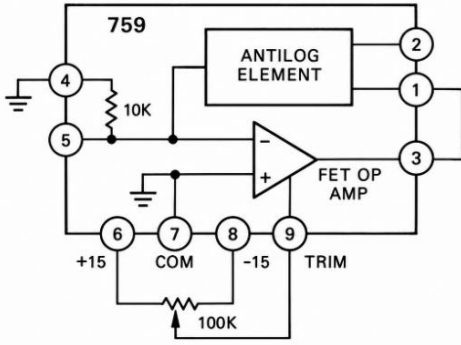
Figure 3. Trimming E_{OS} in Log Mode
