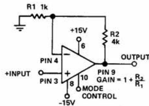
Figure 3. Noninverting Operation
