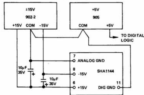
Figure 5. Power Supply and Grounding Connections
