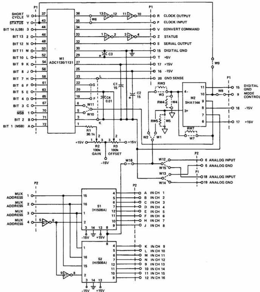
Figure 11. Schematic and Pin Designations
