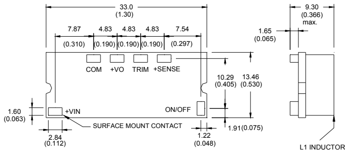
Figure 16. S15-5S3.3 Mechanical Outline Diagram
