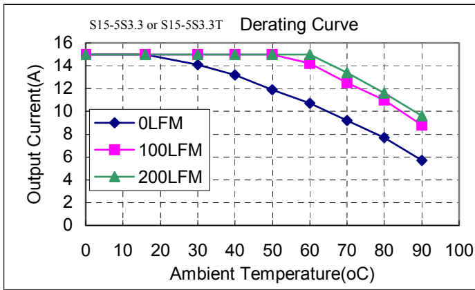
Figure 8. Typical Power De-rating for 5.0V IN (S15-5S3.3)
