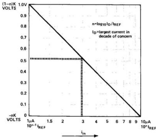
Figure 2. Input vs. Output for Any One Decade of Operation
