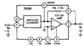
Figure 4. Functional Block Diagram
