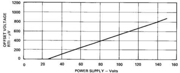
Figure 6. Input Offset Voltage vs. Power Supply Voltage
