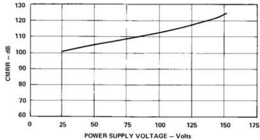
Figure 5. CMRR vs. Power Supply Voltage
