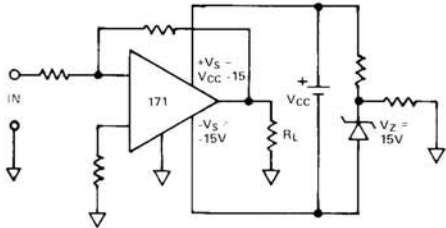
Figure 2. Single Supply Operation
