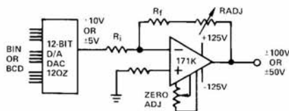
Figure 8. Programmable Power Supply
