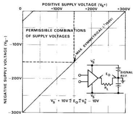
Figure 1. Power Supply Voltage Combinations
