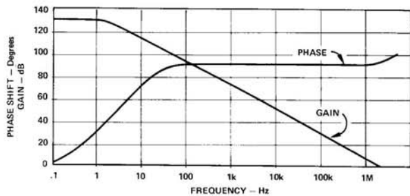
Figure 3. Gain and Phase Shift vs. Frequency
