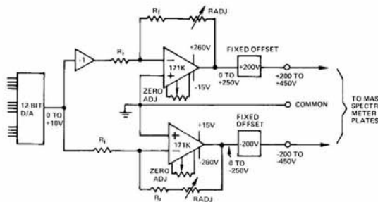
Figure 9. Programmable Mass Spectrometer Voltage Source
