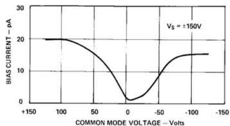
Figure 7. Bias Current vs. CMV for Model 171K
